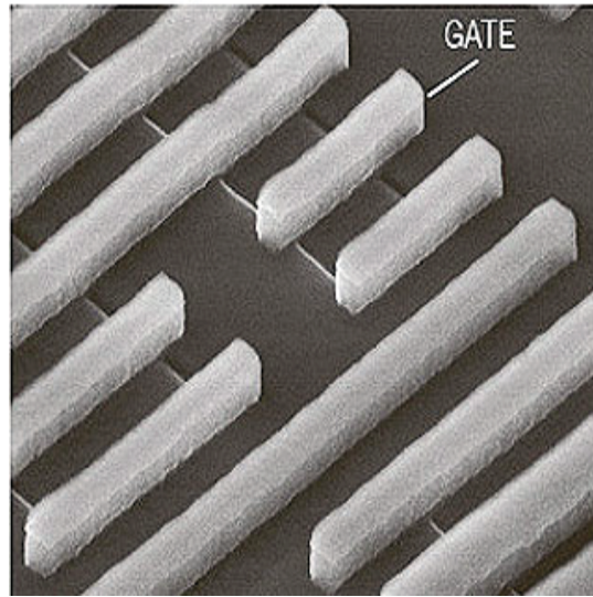
Traditional planar transistor
