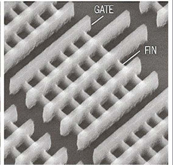
Intel Tri-Gate transistor
